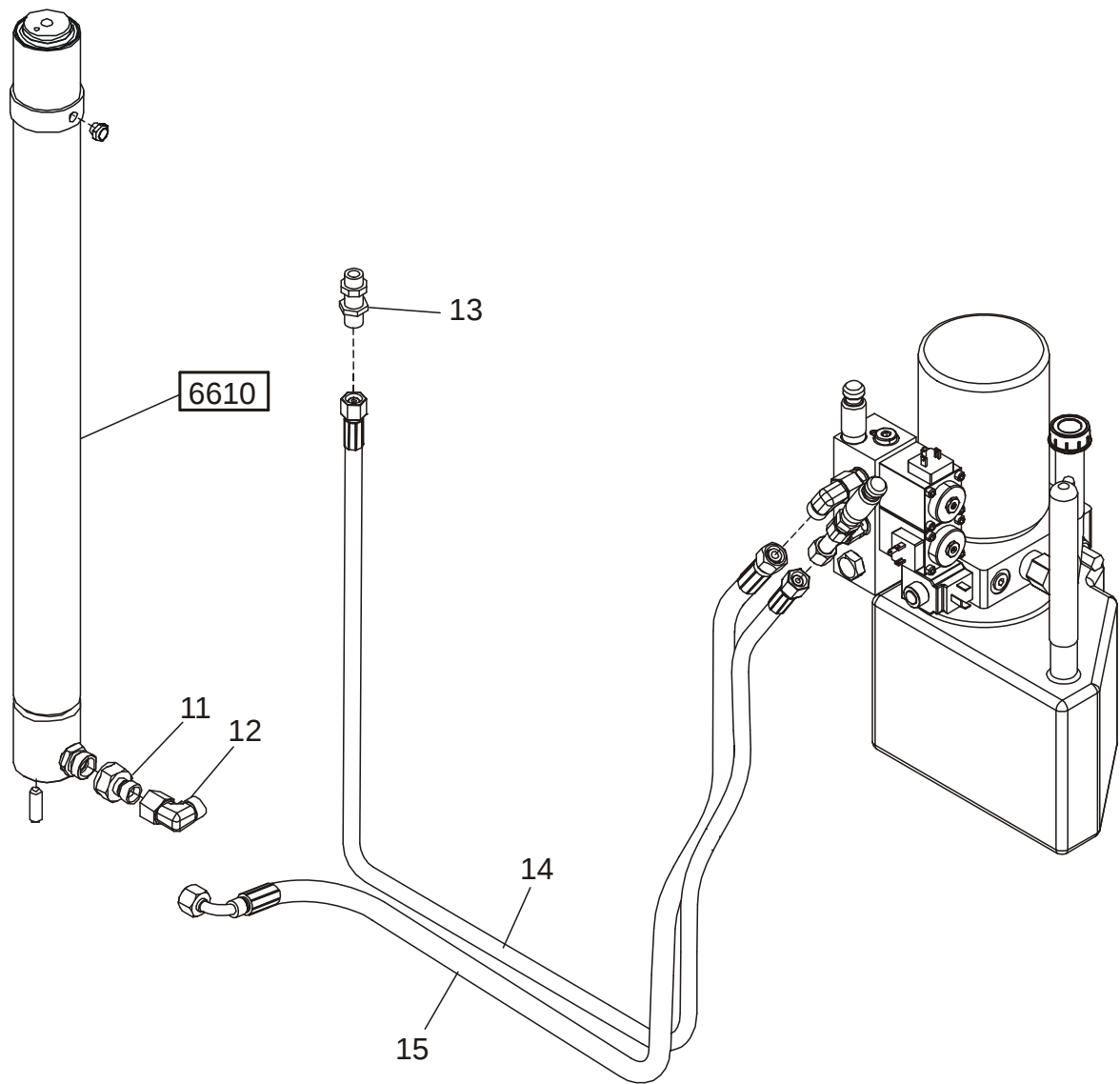
6230-00137 Hydraulic lines chassis [2006-04-07] Chassimonterade hydraulledningar; Hydraulikleitungen Chassis; Circuits hydrauliques châssis;
